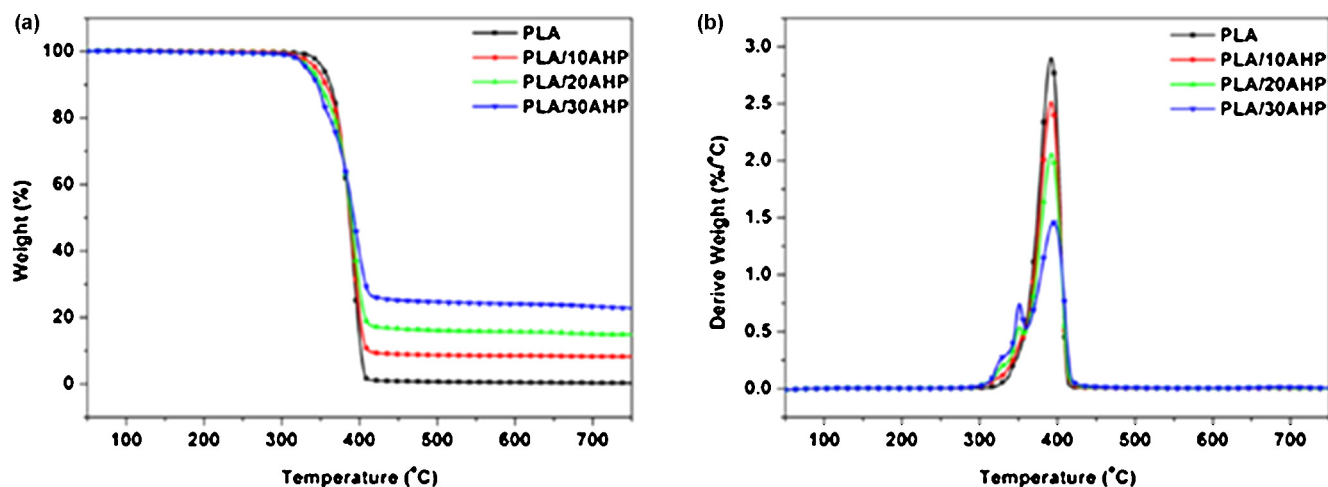
Fig. 18. TGA and DTG curves of PLA and FR-PLA composites under nitrogen condition.
