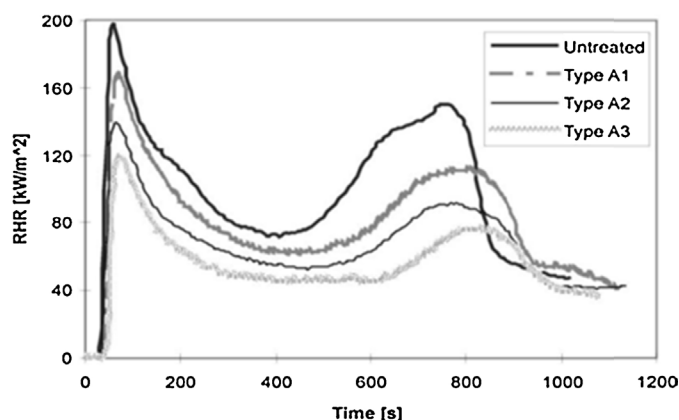
Fig. 2. HRR as a function of time for untreated and FR treated particleboard with the use of magnesium hydroxide.
