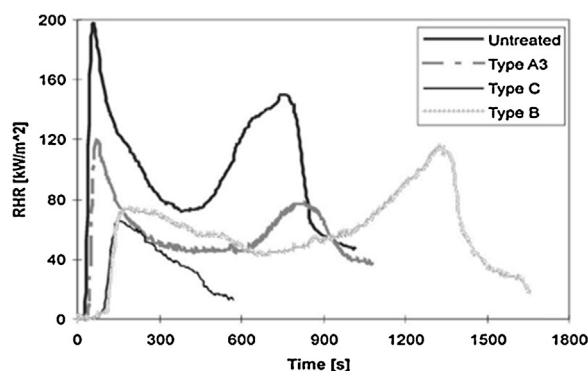
Fig. 10. HRR versus time for untreated and flame retardant treated particle board with the use of different flame retardant combinations.
