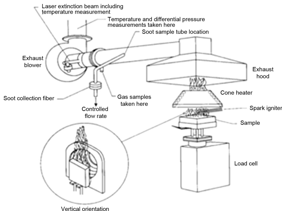
Fig. 4. Schematic representation of an experimental set-up in a cone calorimeter.
