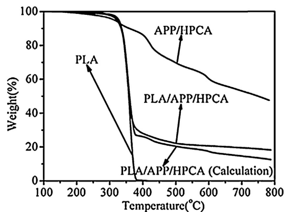
Fig. 15. TGA curves of PLA, APP/HPCA, PLA/APP/HPCA, PLA/APP/HPCA (calculation). Reprinted from Ke et al. (2010), Copyright 2010, with permission from Elsevier.
