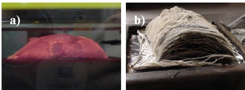
Fig. 12. Images of (a) flax twill weave in a cone calorimeter, and (b) a burnt flax unidirectional fabric sample.
