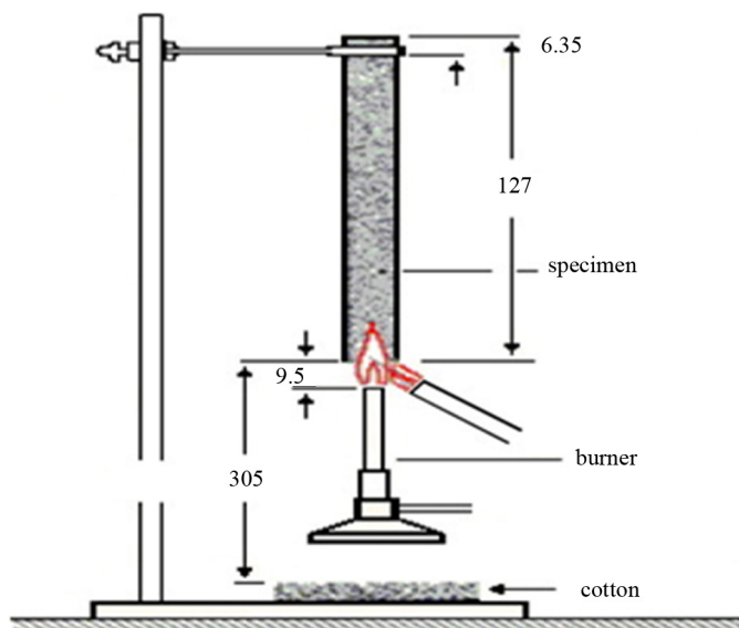
Fig. 7. Schematic representation of UL 94 vertical test. Reprinted from Laoutid et al. (2009), Copyright 2009, with permission from Elsevier.
