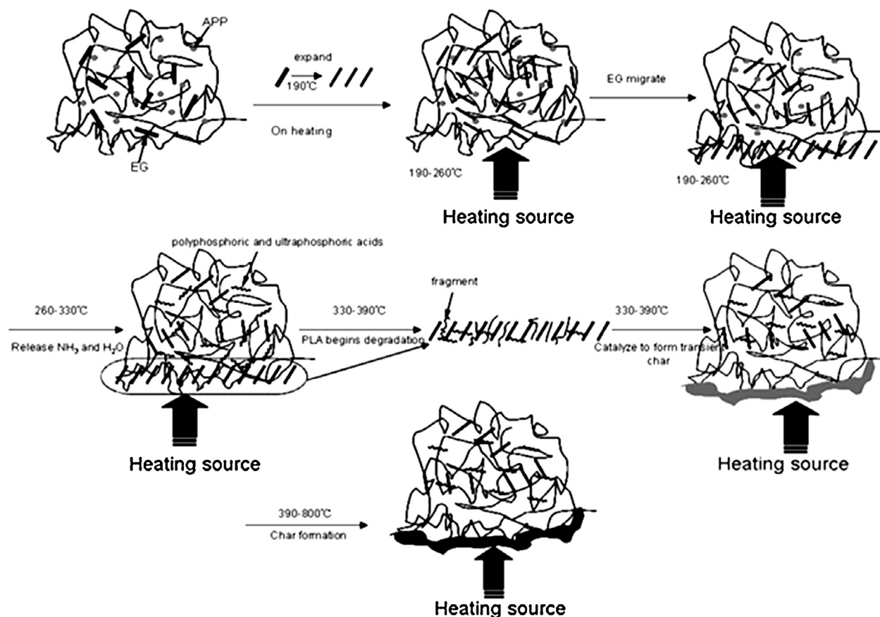
Fig. 17. Possible flame retardant mechanism of PLA/APP/EG composite.
