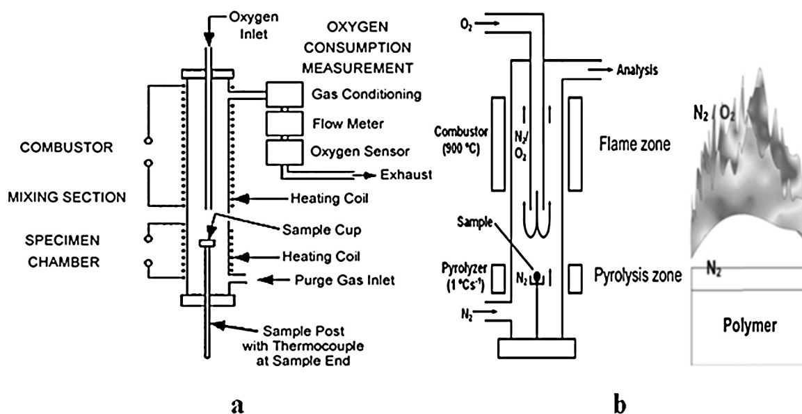
Fig. 5. Schematic representation of pyrolysis combustion flow calorimetry (PCFC): (a) basic section of the apparatus. Reprinted from Morgan et al. (2009), Copyright 2009, with permission from Elsevier. (b) Experimental set-up of the PCFC (left) in comparison with the flaming combustion of a polymer (right). Reprinted from Schartel et al. (2007), Copyright 2007, with permission from Elsevier.
