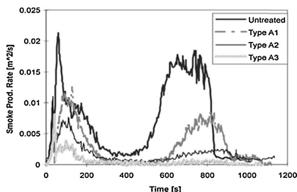
Fig. 9. Smoke production rate versus time for non-treated and magnesium hydroxide-treated particleboard.
