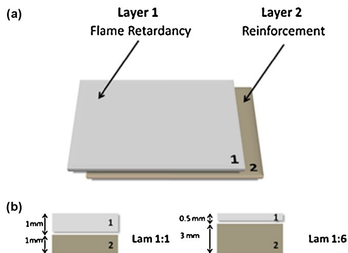
Fig. 20. Structure (a) and laminate thickness (b) of the investigated materials. Reprinted from Gallo et al. (2013), Copyright 2013, with permission from Elsevier.
