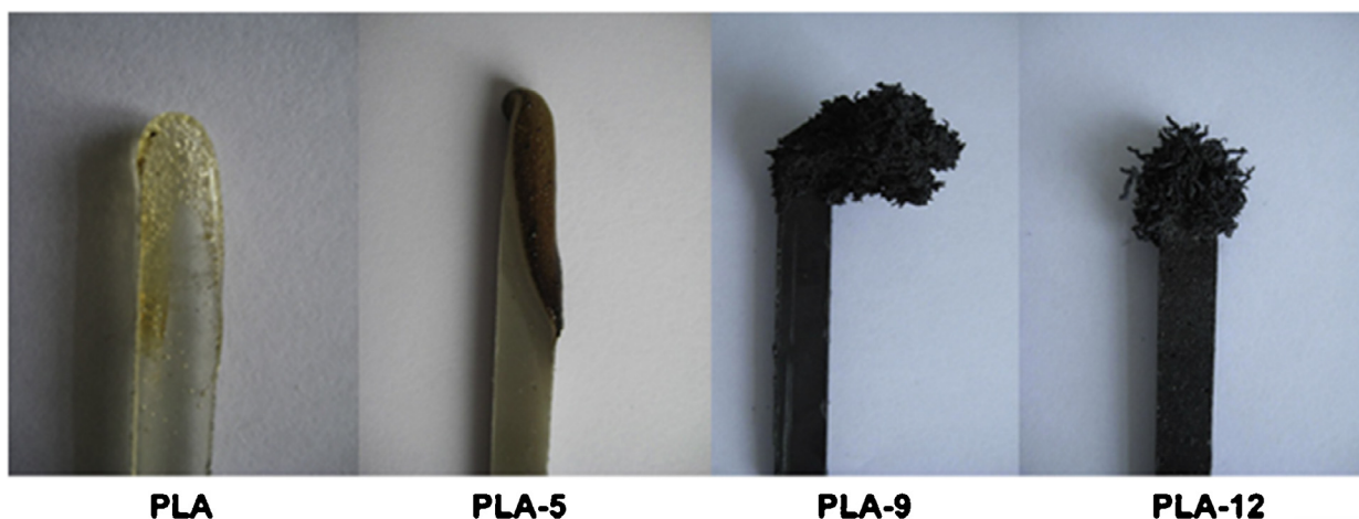
Fig. 14. Photographs of PLA specimens after LOI tests.
