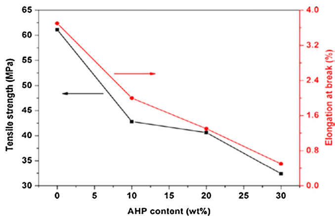
Fig. 19. Effect of AHP loading on the mechanical properties of FR/PLA composites.
