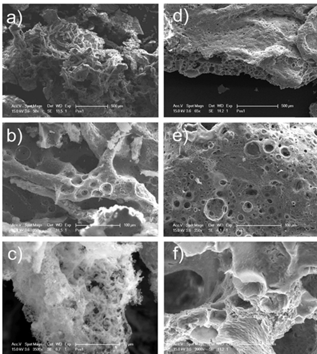
Fig. 22. SEM micrograph of Layer 2 (a–c) and Lam 1:6 (d–f) at different magnifications.
