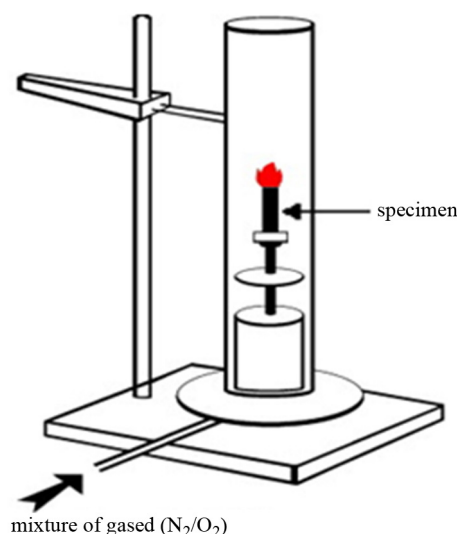
Fig. 6. Schematic representation of a limiting oxygen index (LOI) test setup. Reprinted from Laoutid et al. (2009), Copyright 2009, with permission from Elsevier.
