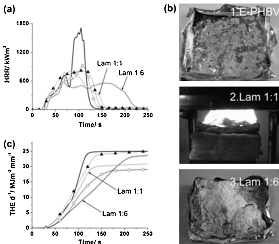
Fig. 21. Heat release rate for E-PHBV (solid line), Layer 1 (open circles), Layer 2 (solid triangles) and laminate structures (a); fire residue after cone calorimeter test for E-PHBV (b.1), barrier formation during burning (Lam 1:1) (b.2) and fire residue for Lam 1:6 (b.3); total heat evolved (c).
