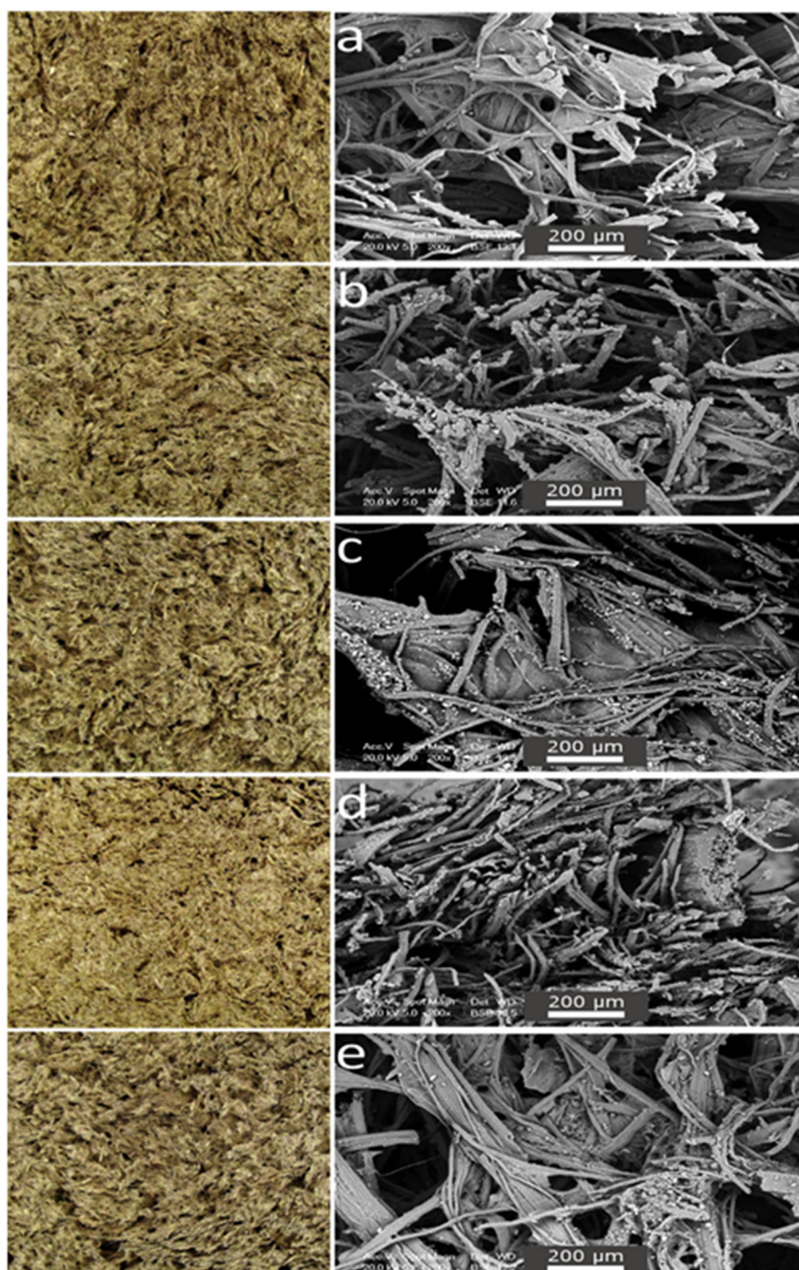
Fig. 11. Macroscopic and SEM pictures ( \times 200 ) of (a) reference (untreated flax fibre), and flame retardant treated flax (fibre and pea protein binder) containing 20 wt.% of (b) ATH, (c) ZB, (d) MMP and (e) MMB.
