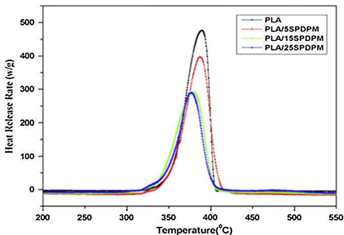
Fig. 16. The HRR curves of PLA and its composites at 1 K/s heating rate. Reprinted from Zhan et al. (2009), Copyright 2009, with permission from Elsevier.
